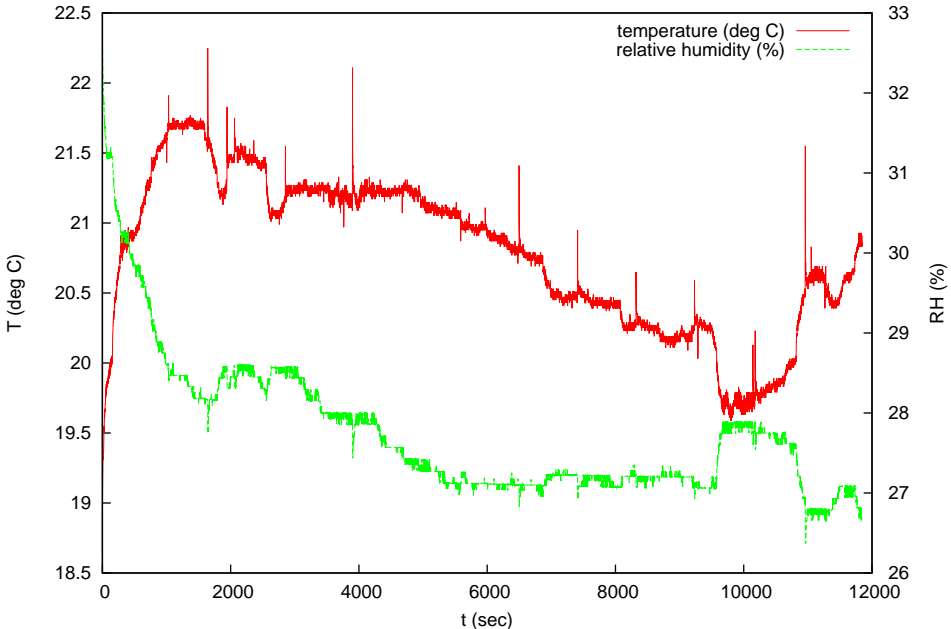
TEMPer Hum test (USB SHT11-based temperature logger)
